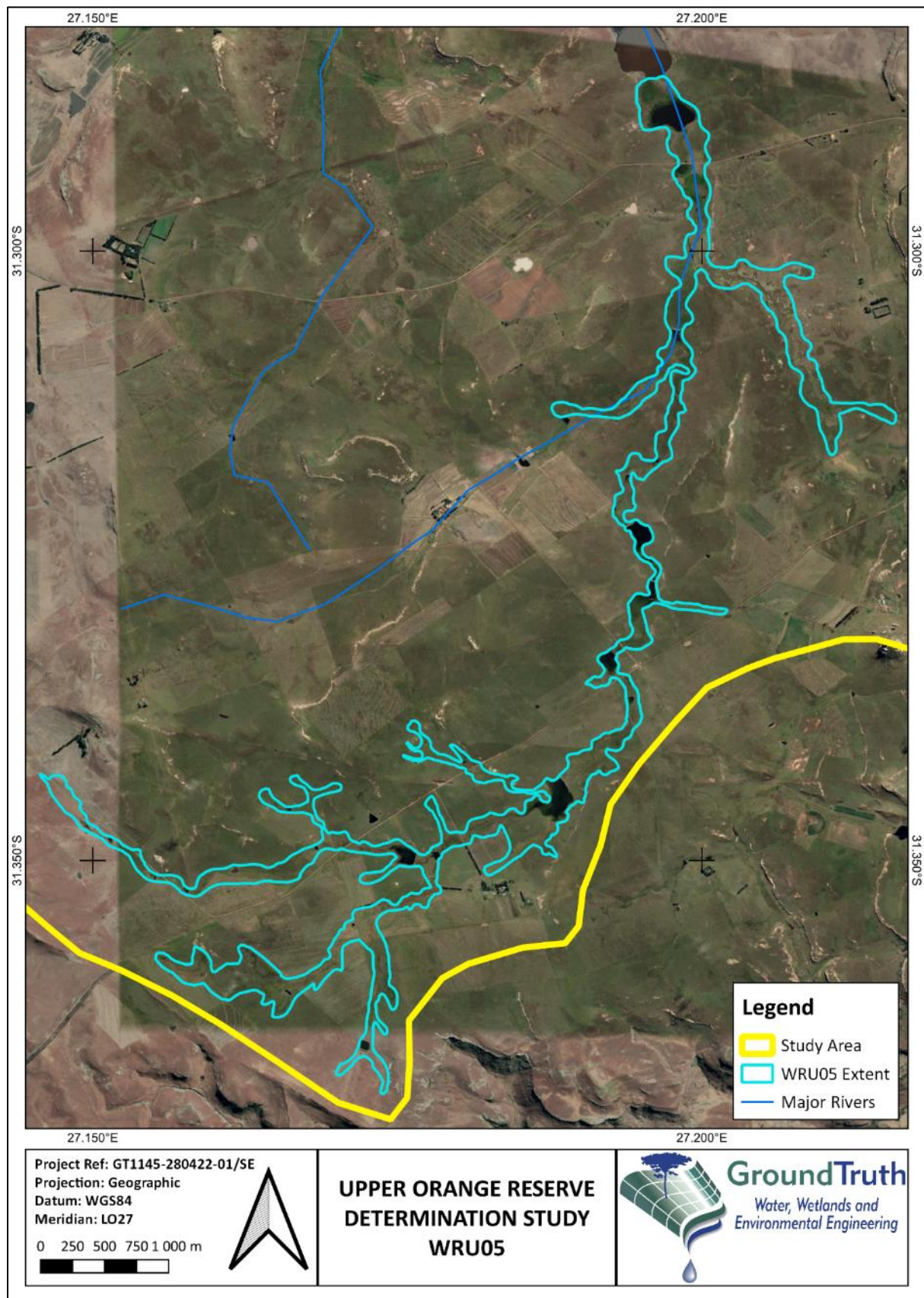
Figure 3-9 Overview of WRU05
